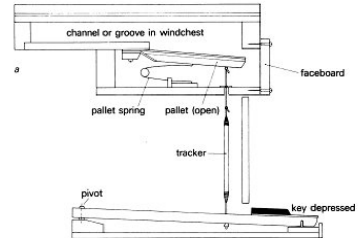
Figure 3 Connections between key and chest:(a)suspended action;the keys are pivoted at the back and hang on the trackers from the pallet valve; (b)detail of the rollerboard
